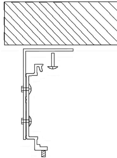
Fig. 1B – Ceiling Mounting
